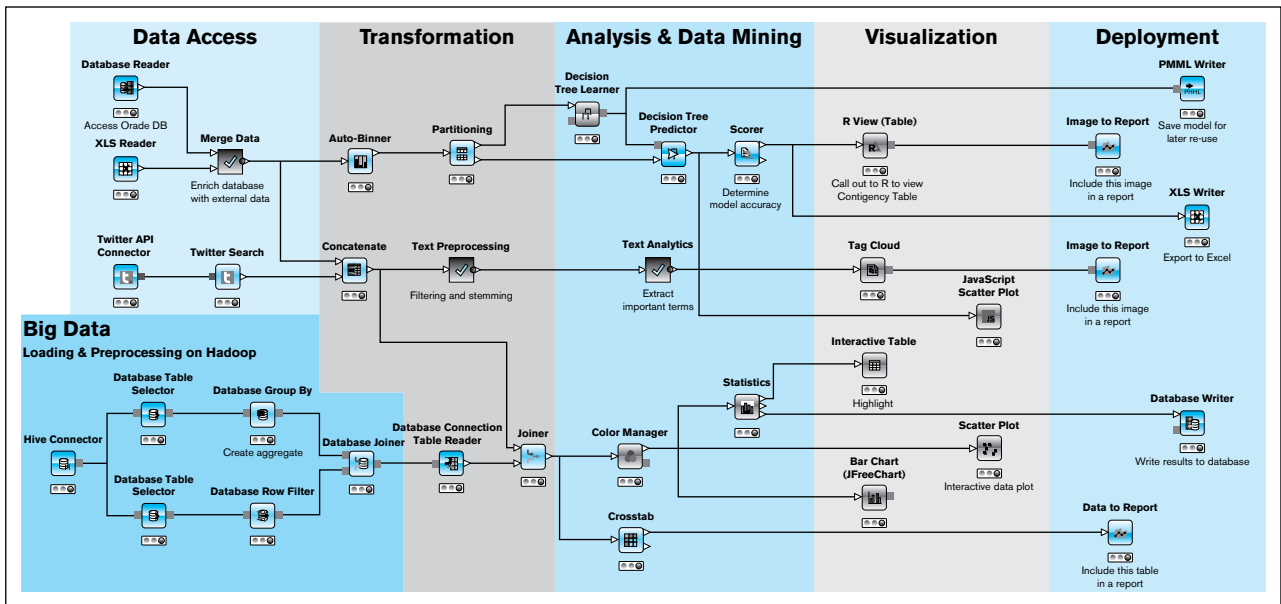
FIGURE 11-17 KNIME architecture
